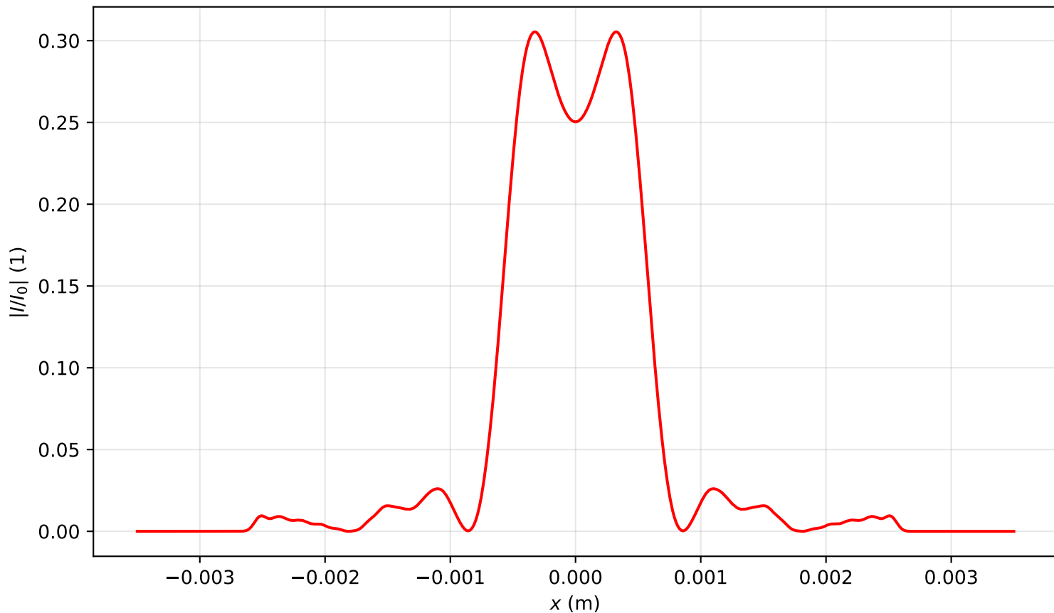
Intensity profile I(x, y = 0, z = 0.955)/I_0 , P_{in}=2.0P_{cr} , artificial time
